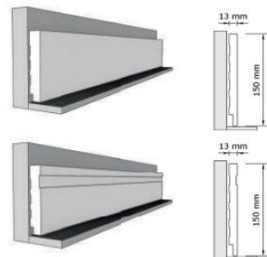
Frisado | 150 x 2400mm
